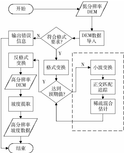
图1 算法流程图 Fig.1 Algorithm flow chart
