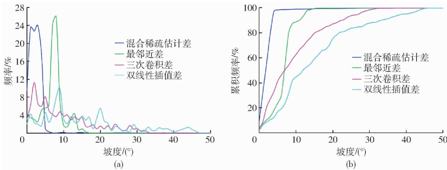
图 7 坡度差值分布的频率及累积频率曲线 Fig. 7 Frequency curves and cumulative frequency curves of slope difference distribution
