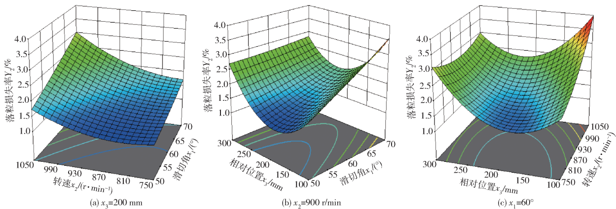
图10 交互因素影响落粒损失率的响应曲面 Fig. 10 Response surface of interaction factors affecting drop loss rate
