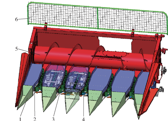
图 1 拨禾链式油葵割台总体结构图 Fig.1 General structure chart of chain oil sunflower harvester header
