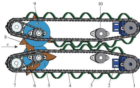
图 2 切割器及动力组成三维图 Fig.2 3D chart of cutting and power composition
