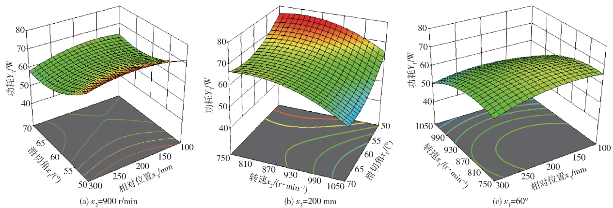
图9 交互因素影响功耗的响应曲面 Fig. 9 Response surfaces with interaction factors affecting power consumption
