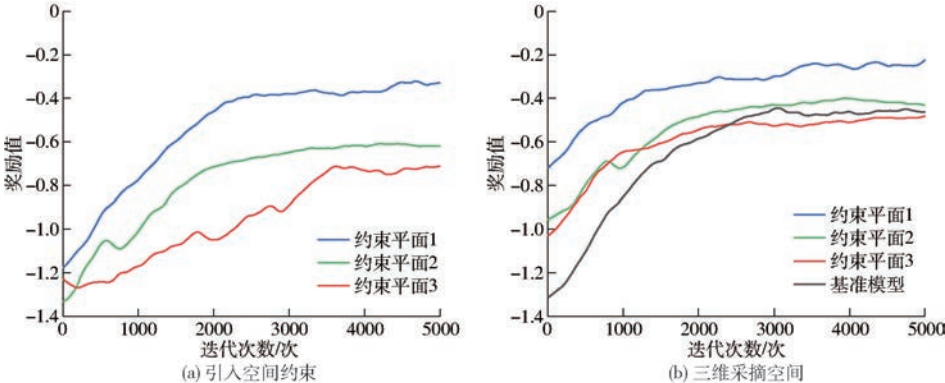
图 10 奖励值变化曲线 Fig.10 Reward value change curves
