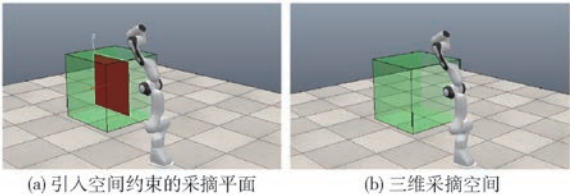
图 2 渐进空间约束分步训练场景 Fig.2 Progressive spatially constrained stepwise training scene
