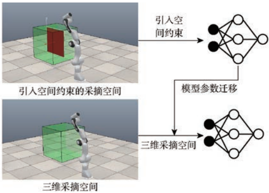
图 3 渐进空间约束分步训练策略流程图 Fig.3 Flow chart of progressive spatially constrained stepwise training strategy
