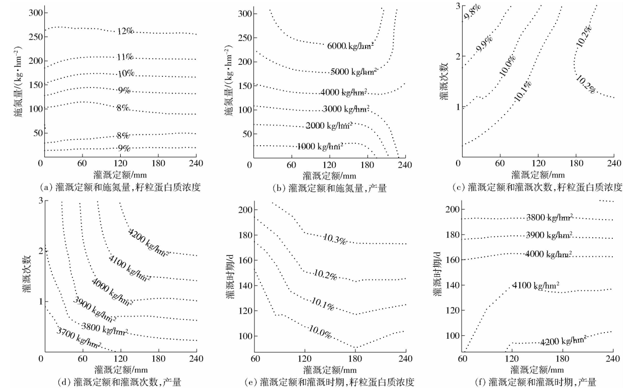
图3 灌溉定额和施氮量耦合、灌溉定额和灌溉次数耦合、灌溉定额和灌溉时期耦合对籽粒蛋白质浓度和产量的影响 Fig.3 Coupling effects of irrigation depth and nitrogen, irrigation depth and irrigation frequency, and irrigation depth and irrigation days after sowing on grain protein concentration and yield
