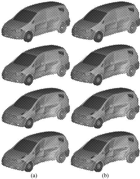
图 3 轻量化前后侧面碰撞整车变形时间历程 Fig. 3 Deformation of car in side impact before and after lightweight (a) 轻量化前 (b) 轻量化后
