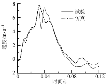
图 9 车身轻量化后整车侧碰试验与仿真速度曲线 Fig. 9 Compare of velocity between experiment and simulation after lightweight in side impact
