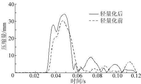
图 7 轻量化前后侧面碰撞假人胸部压缩变形时间历程 Fig. 7 Chest intrusion of occupant in side impact before and after lightweight
