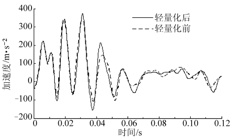
图 4 轻量化前后侧面碰撞 B 柱侧向加速度时间历程 Fig. 4 Side acceleration of B pillar in side impact before and after lightweight
