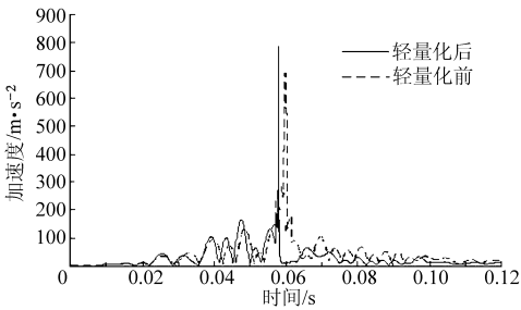
图 6 轻量化前后侧面碰撞假人头部加速度时间历程 Fig. 6 Head acceleration of occupant in side impact before and after lightweight
